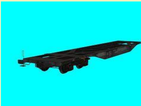
OEBB_Sggmrss-1A-leer_DB1
